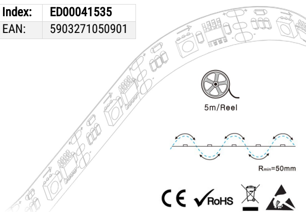
Taśma LED 2835 SMD 120 Neon Side View 12V 10W 26lm/W
