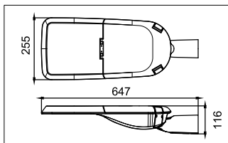
Horizontal installation
