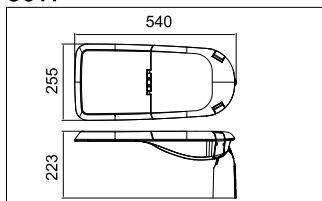
Vertical installation
