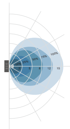
Wall mounting pattern(Unit:m) Suggested installation height: 1-1.8m
