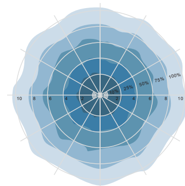
Ceiling mounting pattern(Unit:m) Suggested installation height: 2.5-15m
