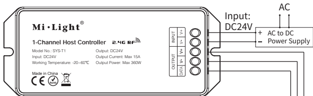
SYS-T1 1-Channel Host Controller (Need to buy separately)
